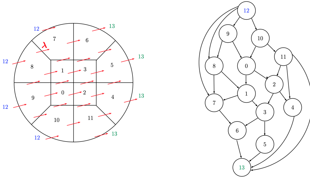
FIGURE 3.2. Left: Unstructured mesh of the disk, with a constant velocity field (in red). The velocity field is chosen to have a slight angle with respect to the horizontal axis to better highlight the dependency between cells. Label 12 represent where up-wind boundary conditions should be provided. Right: Associated dependency graph. Transport is performed from top to bottom nodes.
