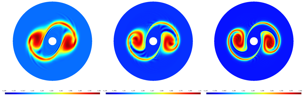
FIGURE 5.6. (Three-dimensional diocotron test case) Density at t_{max} = 100 in the poloidal plane \theta = 0 obtained with n_p = 32 , n_p = 64 and n_p = 128 . Parameters: L = 1 , \rho = 7 , t = 3 , DG order p = 2 , \nu = 1.99 .
