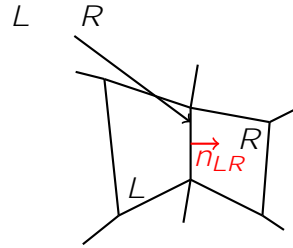
FIGURE 3.1. Normal vector convention.
