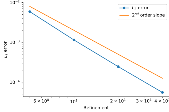
FIGURE 4.3. (Validation in three dimensions) L^2 error as a function of the refinement level. Parameters: t = \rho = 1 , DG order \rho = 2 .
