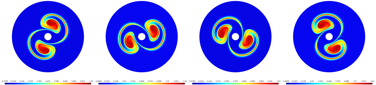
FIGURE 5.4. (Three-dimensional diocotron test case) Density at t_{\max} = 100 for the poloidal planes \theta = 0 , \theta = \frac{L}{4} , \theta = \frac{L}{2} and \theta = \frac{3L}{4} . Parameters: \rho = 7 , t = 600 , DG order \rho = 2 , \nu = 1.99 , n_p = 128 .
