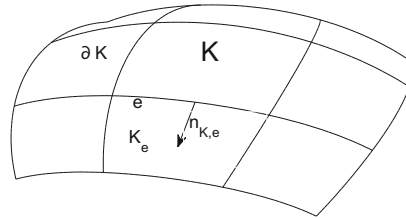
FIGURE 1. Part of a triangulation of the sphere.
