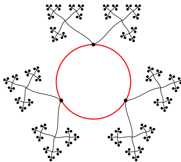
FIGURE 2. The endpoints in the picture is a Cantor set that equals the support of the measure m_{K'} on X^{\text{an}} , where K' is an unramified extension of \mathbb{Q}_2 of degree two.
