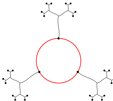
FIGURE 1. The picture shows the Berkovich analytification X^{\text{an}} of the Tate elliptic curve X over \mathbb{Q}_2 defined by (*) . The circle is the Kontsevich–Soibelman skeleton \text{Sk}(X, \theta) , and the three vertices on the circle form the Shilov boundary \text{Sh}(X, \theta) . The measure m_K induced by |\theta| is supported on the Cantor set formed by the endpoints.
