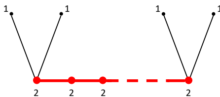
FIGURE 5. The skeleton of the minimal snc -model \mathcal{E} of an elliptic curve E of type I_r^* , r > 0 . The vertices are labeled with the multiplicities of the corresponding components in \mathcal{E}_k . The number of vertices of multiplicity two is r + 1 . The bold part of the graph is \text{Sk}(E, \theta) , for any volume form \theta on E .
