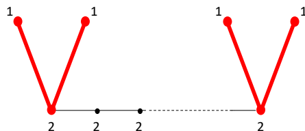
FIGURE 4. The skeleton of the minimal snc-model \mathcal{E} of an elliptic curve of type I_r^* , r \geq 0 . The vertices are labeled with the multiplicities of the corresponding components in \mathcal{E}_k . The number of vertices of multiplicity two is r + 1 (if r = 0 , then the unique vertex of multiplicity two has four adjacent edges). The bold part of the graph is the temperate part \text{Sk}^t(\mathcal{E}) of the skeleton \text{Sk}(\mathcal{E}) if p = 2 .
