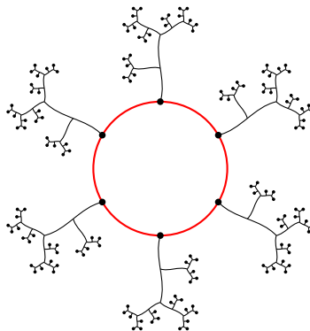
FIGURE 3. The endpoints in the picture is a Cantor set that equals the support of the measure m_{K'} on X^{\text{an}} , where K' is a ramified extension of \mathbb{Q}_2 of degree two.
