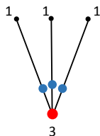
FIGURE 6. The skeleton of the minimal snc-model \mathcal{E} of an elliptic curve E of type IV over K . The vertices are labeled with the multiplicities of the corresponding components in \mathcal{E}_k . The lattice length of each edge is equal to 1/3 . For any volume form \theta on E , the skeleton \text{Sk}(E, \theta) consists of the unique vertex of multiplicity 3, which is wild if p = 3 . The three marked points in the interiors of the edges form the image of the Shilov boundary \text{Sh}(E \otimes_K K', \theta \otimes_K K') where K' is a tame finite extension of K . If we set e = e(K'/K) , then the lattice distance from each point in \text{Sh}(E \otimes_K K', \theta \otimes_K K') to the vertex of multiplicity 3 equals 1/3 - \lfloor e/3 \rfloor/e .
