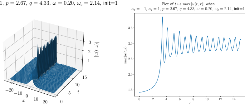
Figure 6. Example of a growing/oscillating numerical solution. The initial data is u^0 = (1 + \varepsilon)\phi_\omega , \varepsilon = 10^{-2} .
