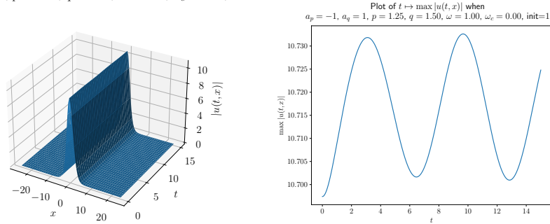
Figure 5. Example of a stable numerical solution. The initial data is u^0 = (1 + \varepsilon)\phi_\omega , \varepsilon = 10^{-2} .
