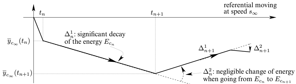
FIGURE 2. A schematic picture of the broken line in the (t, y) -plane which is used in the proof of Proposition 7.1. The main idea is to control the energy decay along the straight sections, as well as the small energy variations occurring at the vertices.
