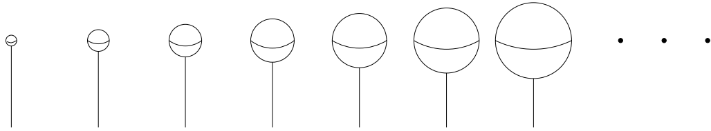
FIGURE 2. The balloon space \mathcal{B}^n , with infinite whiskers attached to each sphere.
