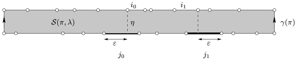
FIGURE 6. A separatrix of length 2 (here the canonical separatrix \gamma(\pi) has length 1). The two corresponding horizontal intervals of lengths \lambda_{j_0+r} and \lambda_{j_1+r} , labelled by j_0 and j_1 , are glued by a central symmetry.
