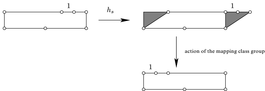
FIGURE 4. Action of the horocyclic flow h_s on a flat surface.
