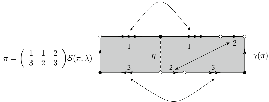
FIGURE 3. A suspension over a permutation \pi with an appropriate admissible vector \lambda . The resulting point (\mathcal{S}(\pi, \lambda), dz^2) belongs to the stratum \mathcal{Q}(-1, -1, 2) . The black bullets correspond to the poles and the white bullets to the unique zero of the differential q on \mathcal{S}(\pi, \lambda) .
