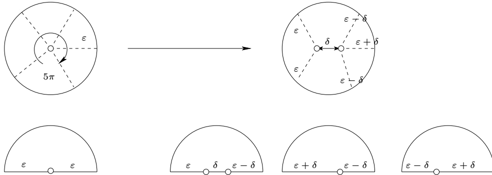
FIGURE 1. Breaking up a zero of order 3 in two zeroes of orders 1 and 2 correspondingly. Note that the surgery is local: we do not change the flat metric outside of the neighborhood of the zero.
