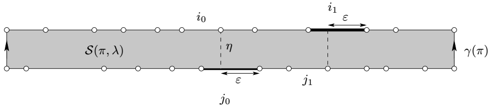
FIGURE 5. A separatrix of length 2 (here the canonical separatrix \gamma(\pi) has length 1). The two corresponding horizontal intervals of lengths \lambda_{j_0+r} and \lambda_{i_1} , labelled by j_0 and i_1 , are glued by a translation.
