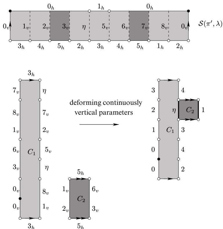
FIGURE 12. A flat surface \mathcal{S}' = \mathcal{S}(\pi' \lambda_0) suspended over the permutation \pi' and the admissible vector \lambda_0 (see Equation (7.1)). The vertical foliation decomposes \mathcal{S}' in two cylinders C_1 and C_2 . The cylinder C_2 is a simple cylinder: the conical angle of its boundary \eta is \pi . Moreover the length of \eta can be chosen arbitrary small with respect to other vertical parameters: C_2 has multiplicity one.
