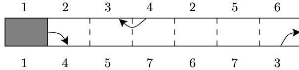
FIGURE 8. A vertical decomposition on a flat surface representing the component \mathcal{Q}^{\text{irr},I}(12) .
