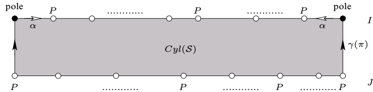
FIGURE 11. A flat surface with a unique zero and a unique pole.
