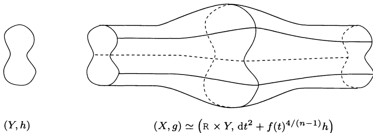
Figure 2. A manifold with many embedded eigenvalues: f(t) large on a compact set.
