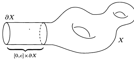
Figure 1. A manifold with a cylindrical end.
