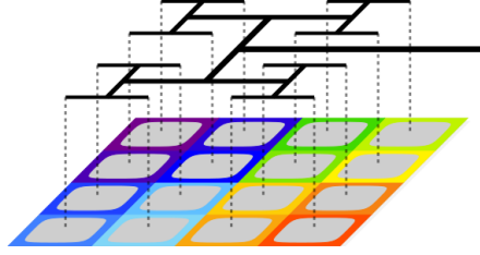
FIGURE 6. H-Tree
