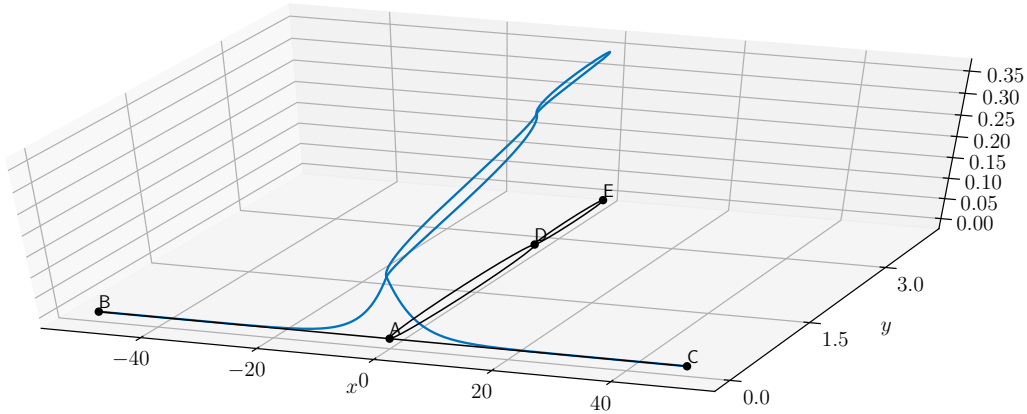
Figure 5.13. The numerical ground state on the tower of bubbles graph
