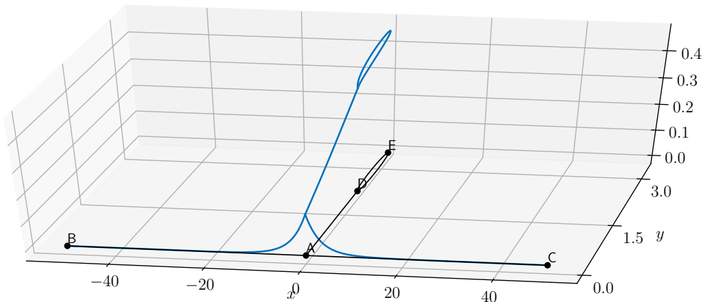
Figure 5.11. The numerical ground state on the signpost graph
