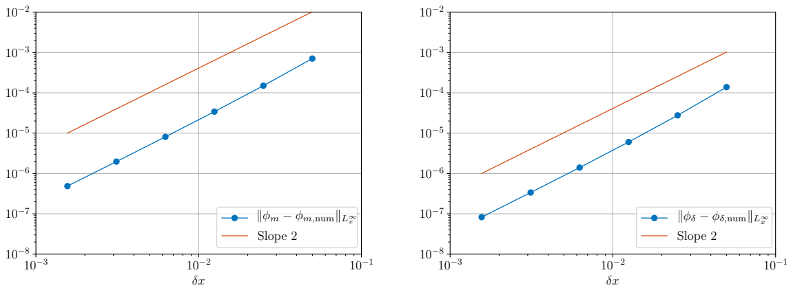
Figure 5.7. Convergence curves for Kirchhoff (left) and \delta (right) conditions.
