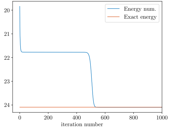
(b) Asymmetric solution, \omega = 16
