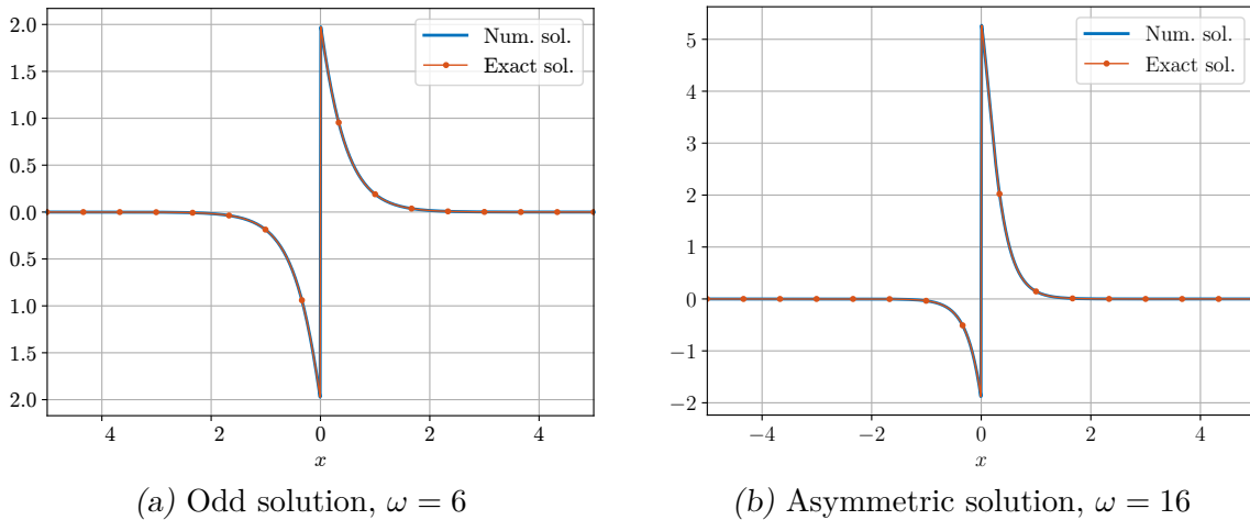
Figure 5.8. Comparison of numerical solutions to ground states for \delta' interaction, \beta = 1
