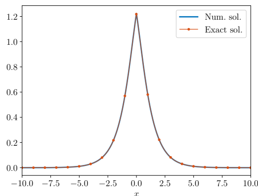
Figure 1.3. Comparison of numerical solution to ground state for \delta interaction.
