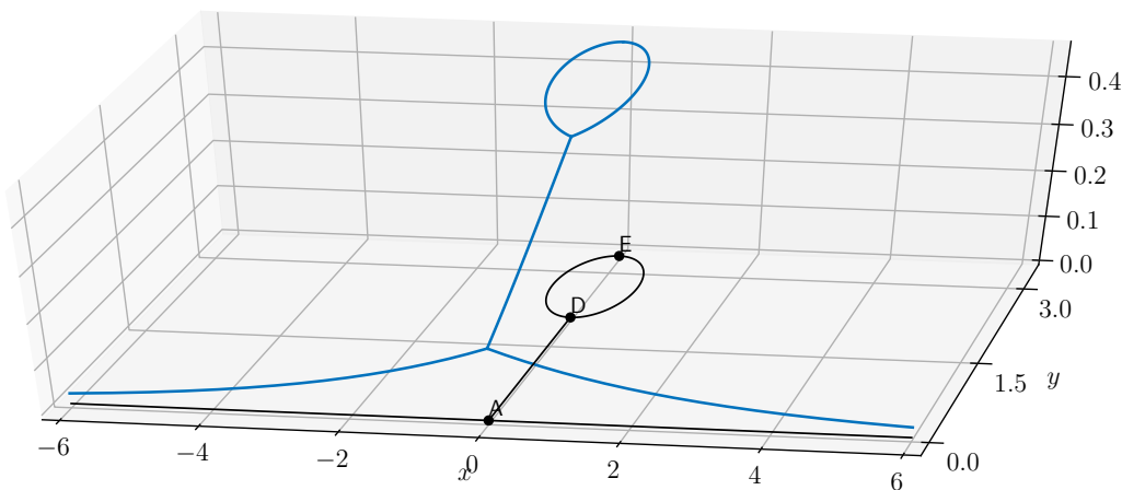
Figure 5.12. Zoom of the numerical ground state on the signpost graph
