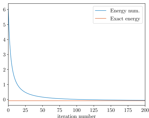
Figure 5.4. Evolution of the energy when computing the ground state of (5.1) for x \in \mathbb{R} compared to E_{NLS} .
