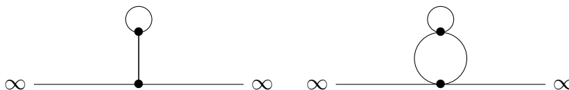
Figure 2.2. Line with a signpost graph (left) and with a tower of bubbles (right).
