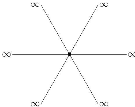
Figure 1.1. Star-graph with N = 6 edges
