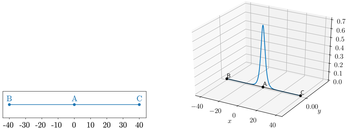
Figure 5.2. Two-edges graph (left) and the exact solution \phi_m(x) for m = 2 (right)
