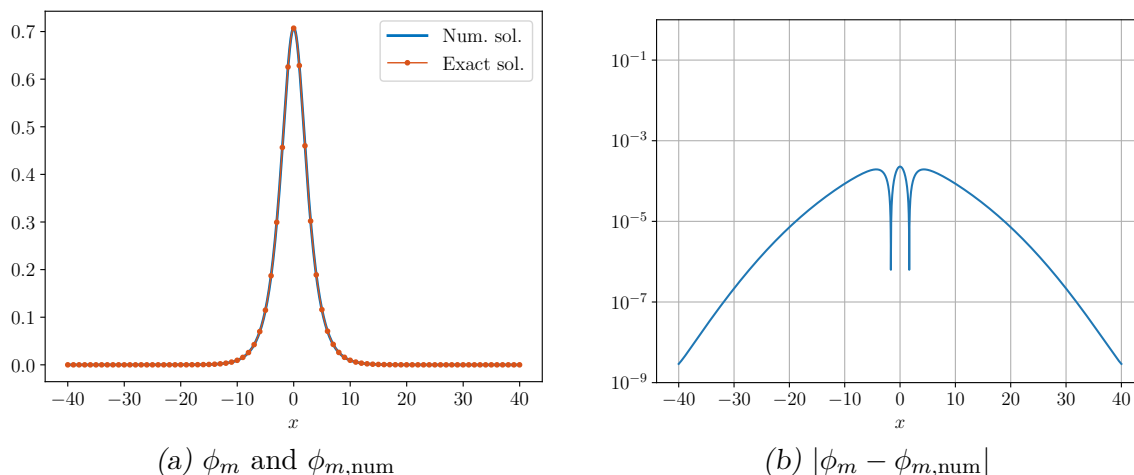
Figure 5.3. Comparison between \phi_m and \phi_{m,num}
