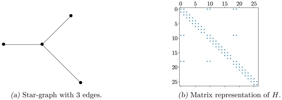
Figure 4.2. An example for a star-graph.
