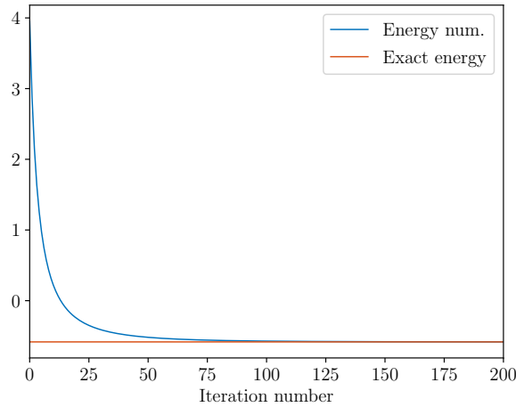
Figure 5.6. Evolution of the energy when computing the ground state of (5.1) with \delta condition compared to E_\delta .
