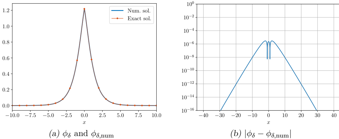
Figure 5.5. Comparison of \phi_\delta and \phi_{\delta,\text{num}} for \delta interaction, \omega = 1 and \alpha = -1 .
