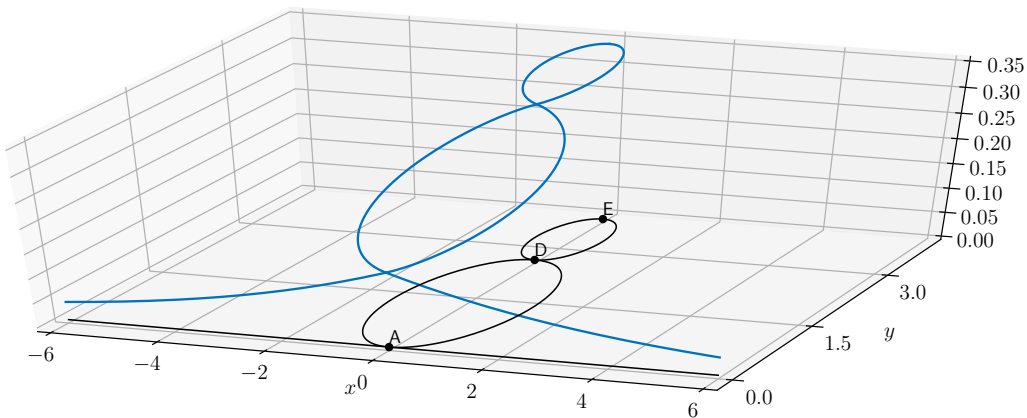
Figure 5.14. Zoom of the numerical ground state on the tower of bubbles graph
