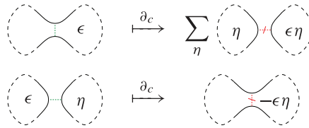
Figure 3. Modified rules for labelling in the differential: here, \epsilon and \eta are element of \{-, +\} and the product is the obvious one.
