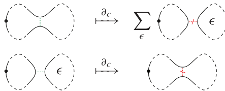
Figure 8. Extra rules for labelling in the reduced differential: here \epsilon is an element of \{-, +\} .
