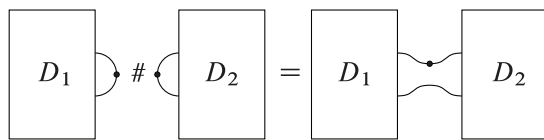
Figure 9. Connected sum for pointed links.
