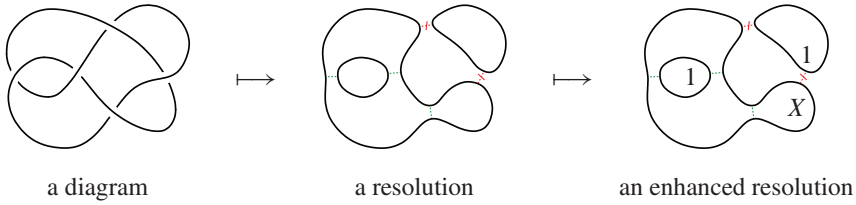
Figure 1. From diagrams to enhanced resolutions.
