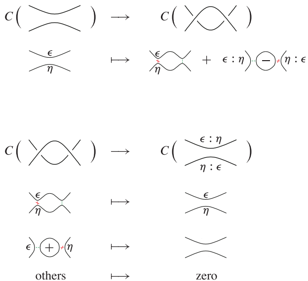
Figure 6. Invariance chain maps: Reidemeister move R2.
