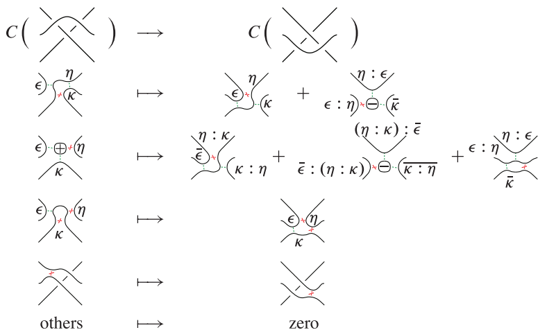
Figure 7. Invariance chain maps: Reidemeister move R3.
