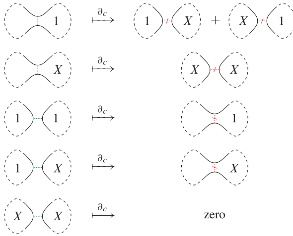
Figure 2. Rules for labelling in the differential: here (and throughout the paper), only the modified part is depicted, the rest of the resolutions being identical on both sides of the arrows.
