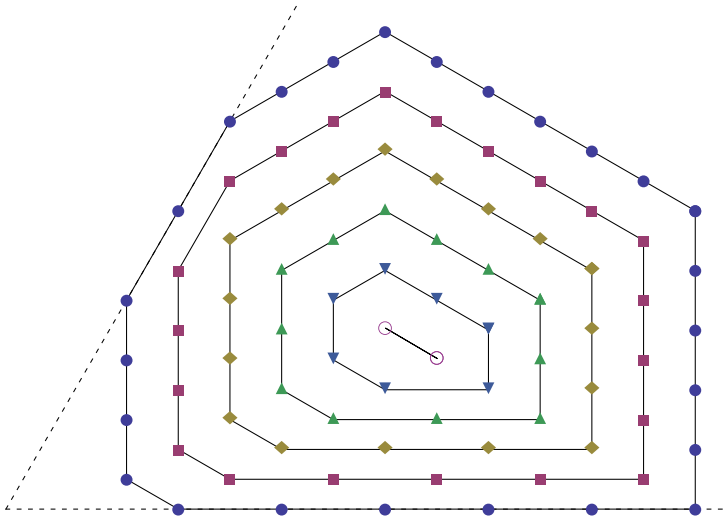
Figure 1. The Horn tensor polytope \tilde{\mathbf{H}}_{\alpha\beta} = \mathbf{H}_{\lambda\mu} for the two SU(3) weights \lambda = (9, 5) \mu = (6, 5) , hence \alpha = (14, 5, 0) , \beta = (11, 5, 0) . The multiplicity increases from 1 to 6 inside the polytope, giving a matriochka pattern to the successive contours.
