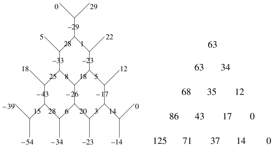
Figure 3. One of the 367 pictographs associated with ((21, 13, 5), (7, 10, 12); (20, 11, 9)) . For completeness we also give below the corresponding KT-honeycomb and its dual hive.
