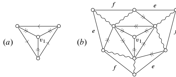
FIGURE 8. Case v_1 \in Z_6
