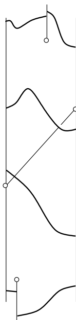
FIGURE 7.1. The vertical strip \mathcal{U} minus rays R_\sigma immerses isometrically in S .
