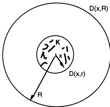
Figure 2 : Elimination Lemma
