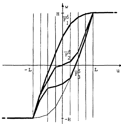
Figure 9. — Piecewise linear monotone curves in the (u, w) -plane corresponding to the graphs B_1 , B_2 and B_3 shown in figure 8, in the case \mu = \text{Lebesgue measure} .
