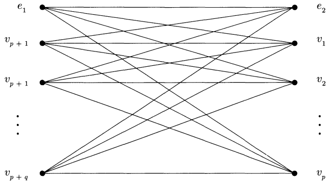
Fig. 11. Graph \mathbf{G}
