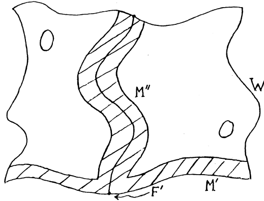
Fig. 1. — An equivariant spin cobordism. The first step puts an invariant metric on the “upper boundary” M'' of the shaded region.
